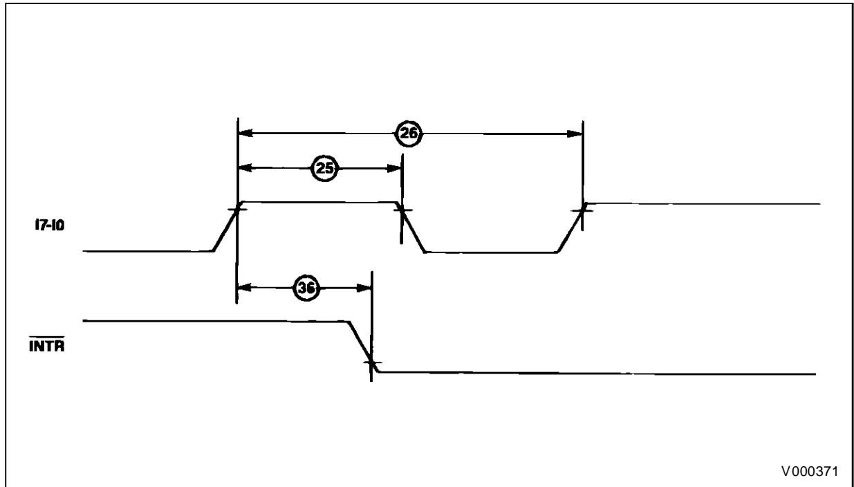
Figure 25 : Interrupt Timing.
