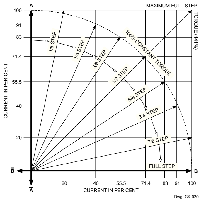
Figure 2 — Current/Displacement Vectors
