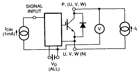
Figure 3 V_{EC} Test
