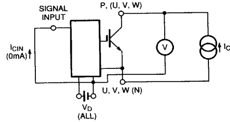
Figure 2 V_{CE(SAT)} Test
