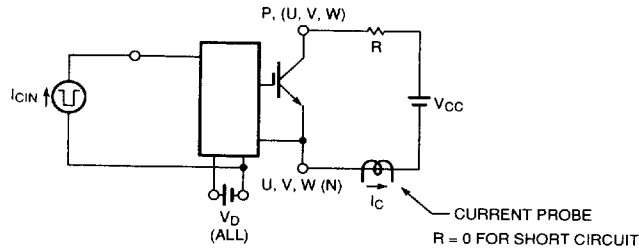
Figure 7 Over Current and Short Circuit Test
