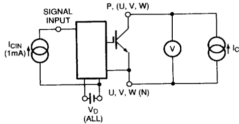
Figure 1 V_{CES} Test
