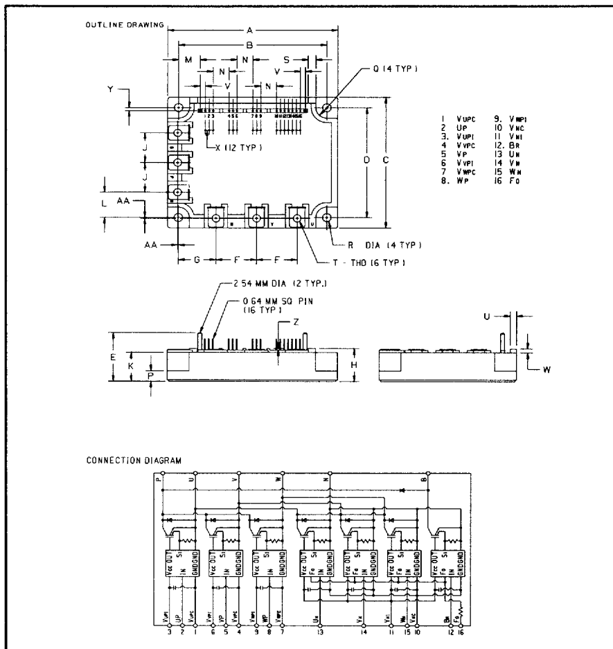
110-230 Volt Line, PM75RHA060 Outline Drawing
