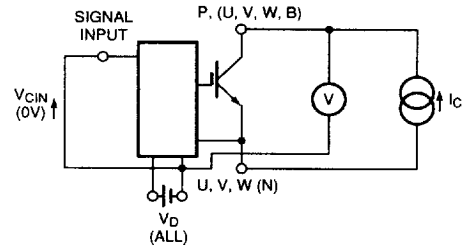
Figure 2 V_{CE(SAT)} Test
