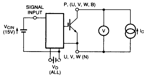
Figure 1 V_{CES} Test
