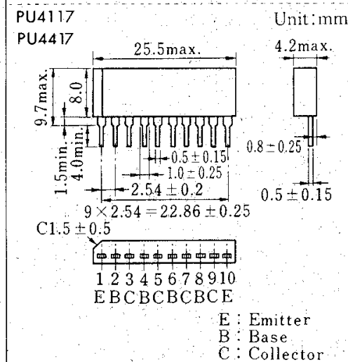
10-Lead Plastic SIL Package
