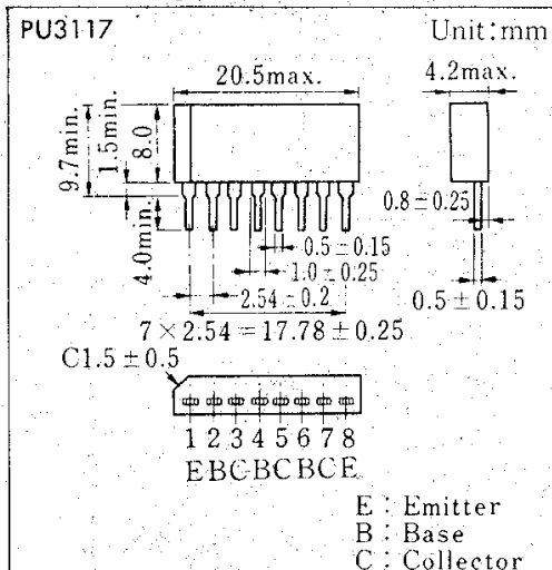
8-Lead Plastic SIL Package
