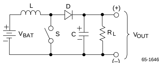
Figure 6. Simple Set-Up
