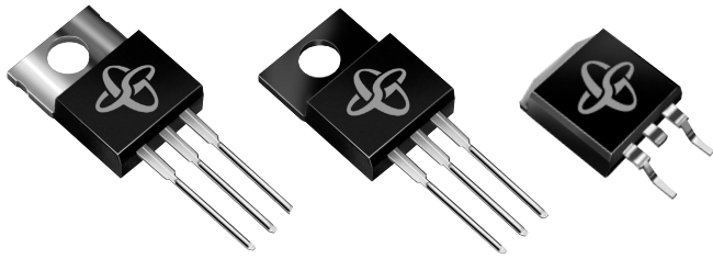
TO-220AB (SBL16xxCT)
