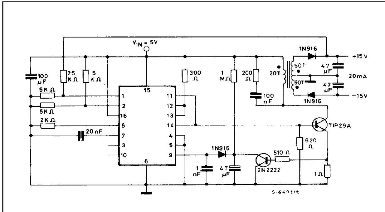
Figure 7: Flyback Converter Circuit.
