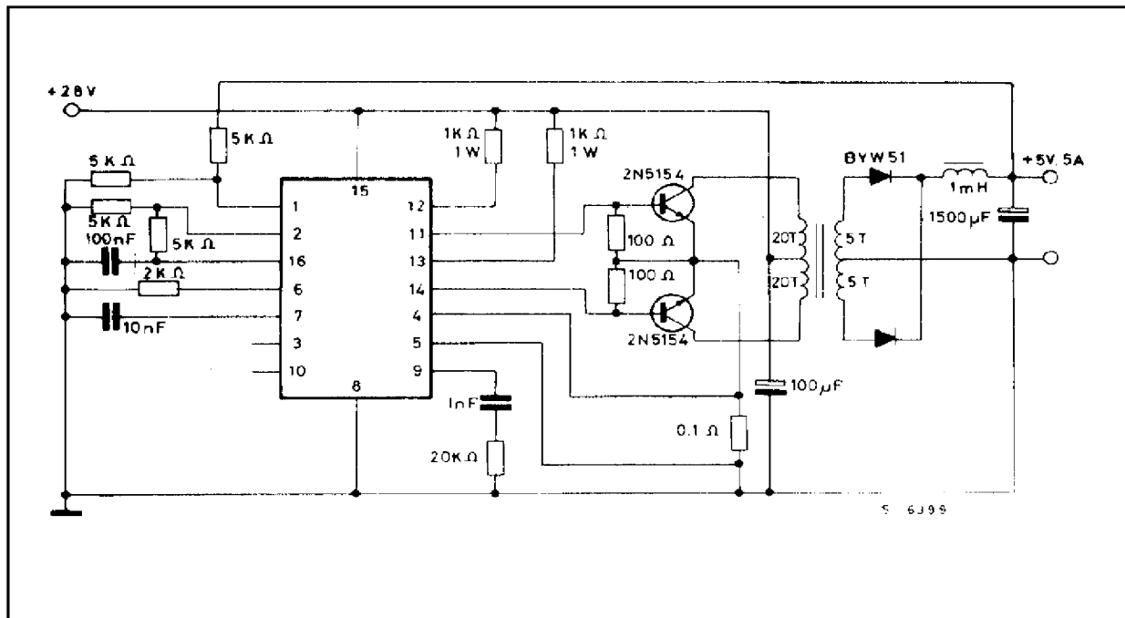
Figure 8: PUSH-PULL Transformer-coupled circuit.
