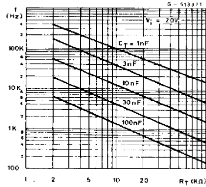
Figure 2: Oscillator Frequency vs. Timing Components
