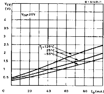
Figure 4: Output Saturation Voltage vs. load Current
