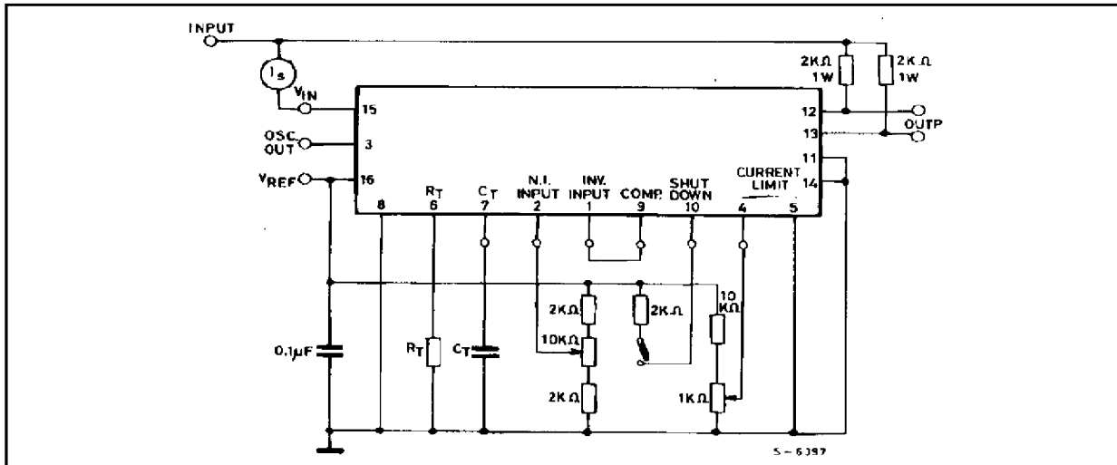
Figure 5: Open Loop Test Circuit.
