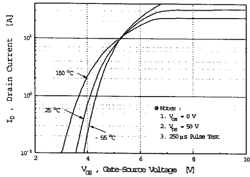
Fig 2. Transfer Characteristics
