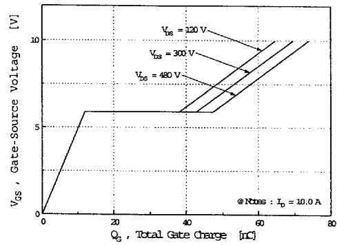
Fig 6. Gate Charge vs. Gate-Source Voltage
