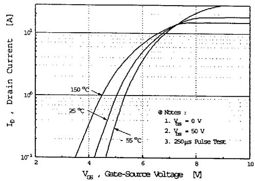
Fig 2. Transfer Characteristics
