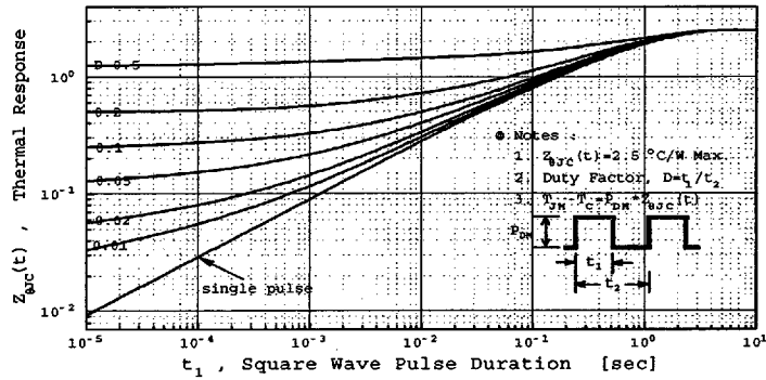
Fig 11. Thermal Response
