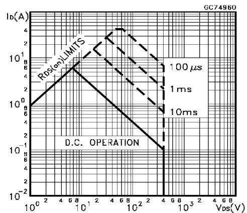
Safe Operating Area for TO-220FP
