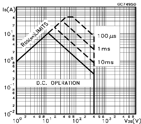
Safe Operating Area for TO-220
