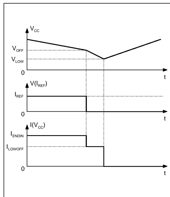
Figure 3 : IC from ON to OFF
