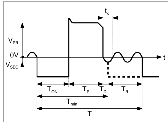
Figure 1 : V_{PRSEC} Voltage Waveform
