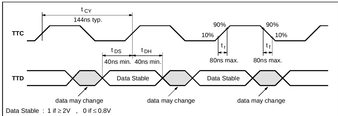
Figure 3 : Synchronization Timing
