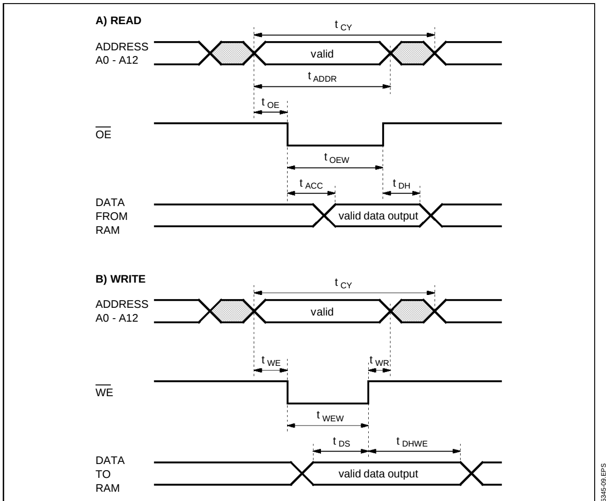
Figure 7 : Memory Interface Timing
