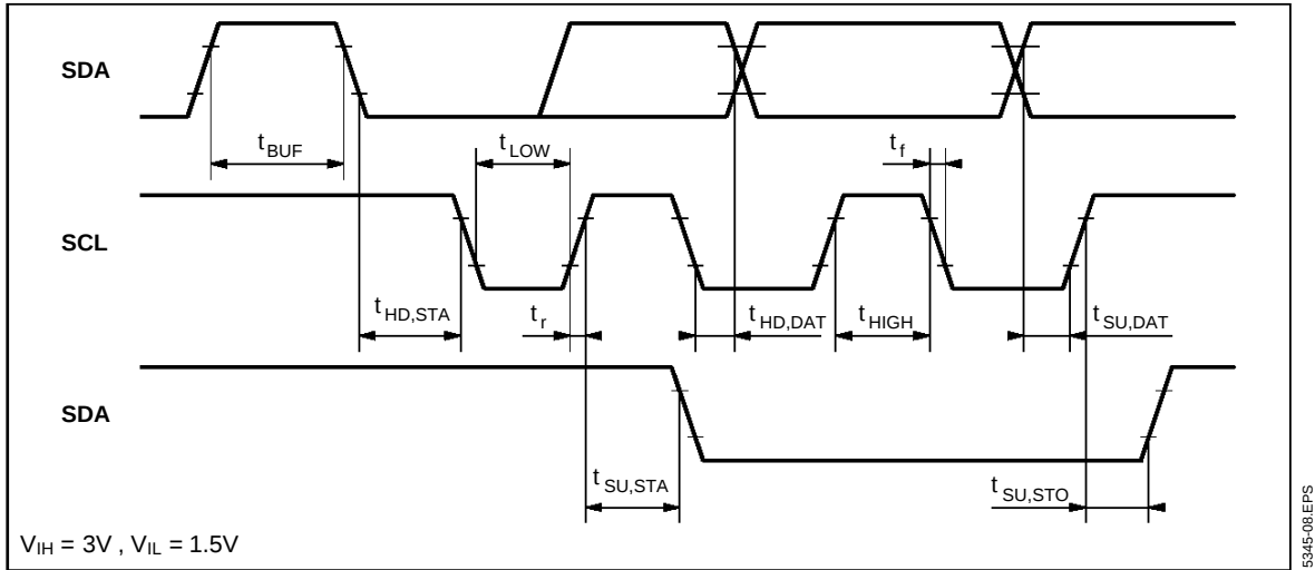
Figure 7 : Memory Interface Timing
