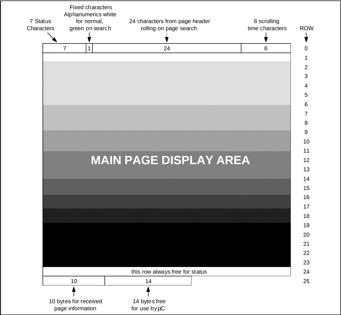
PAGE MEMORY ORGANISATION Figure 10
