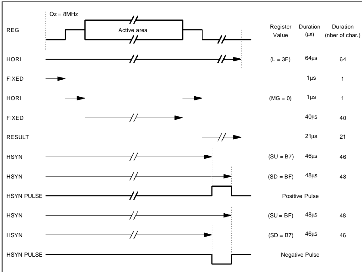
Figure 7 : HSYN Register Synchro Pulse Programming
