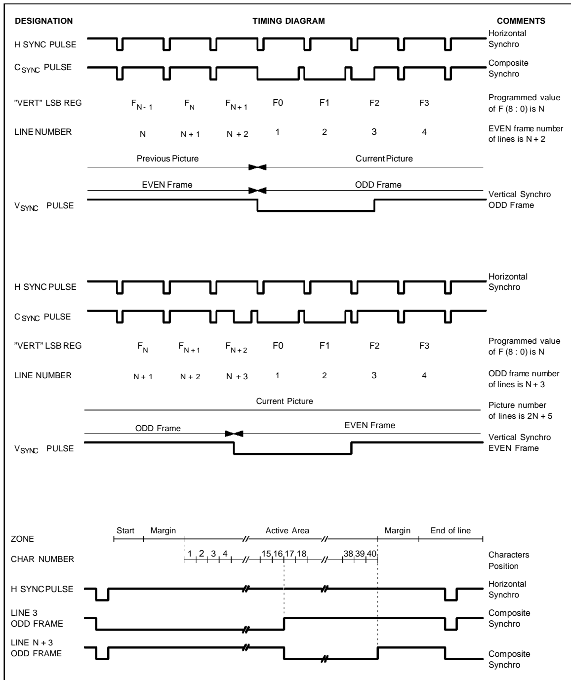
Figure 10 : Interlaced Mode Synchronization Pulses
