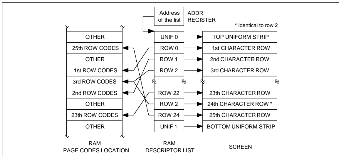
Figure 14 : Relation between Screen Location/Descriptor Pointer/RAM Page Codes
