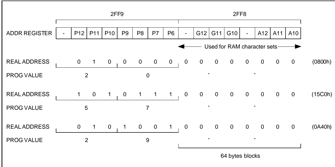
Figure 12 : ADDR Register and Descriptor List Address
