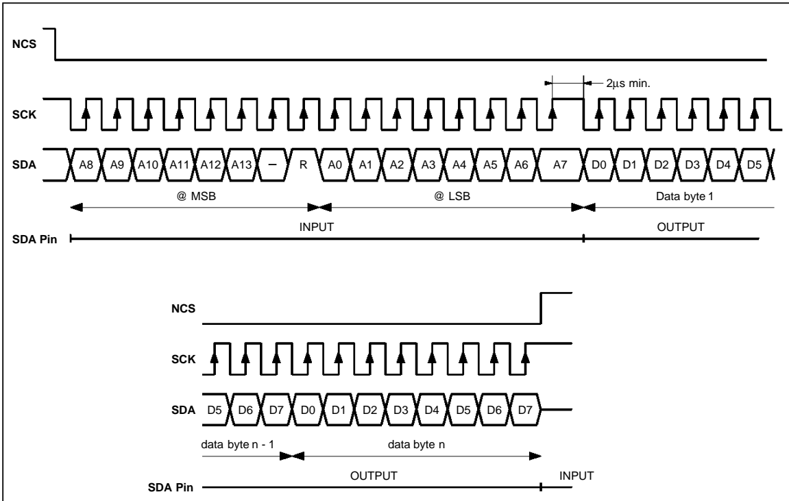
Figure 5 : Serial Interface Read Mode
