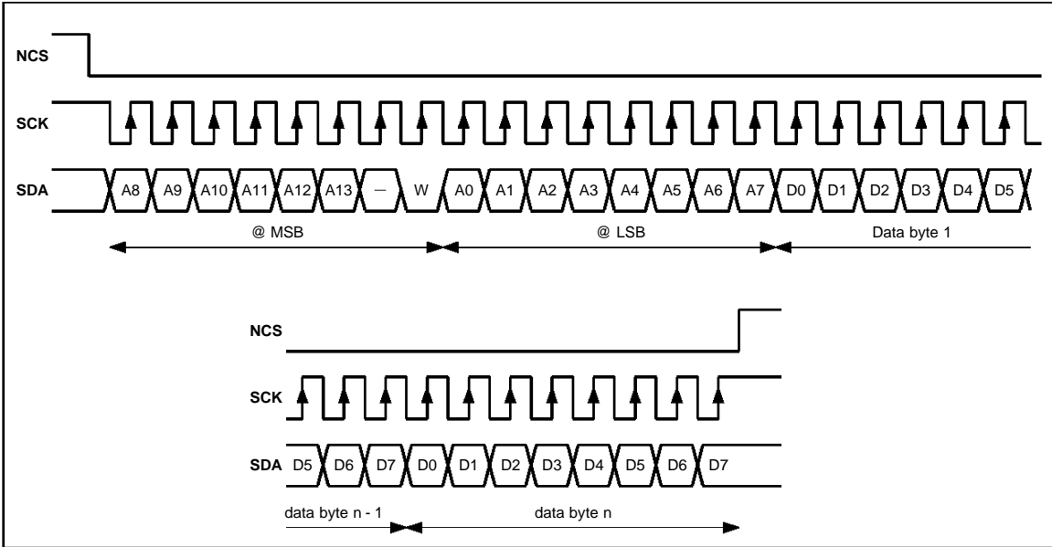
Figure 5 : Serial Interface Read Mode
