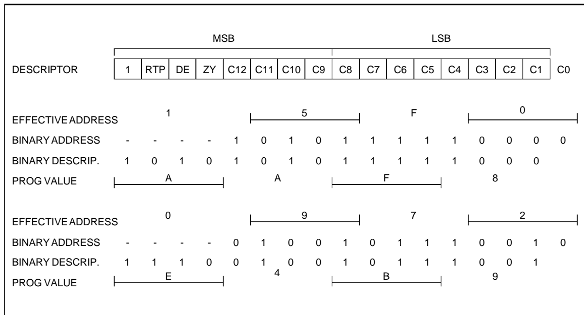
Figure 15 : Character Strip Descriptor - First Character Address Selection
