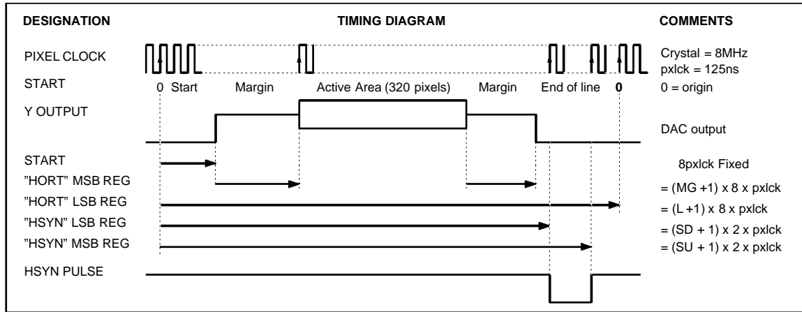
Figure 8 : Horizontal Synchronization Timing
