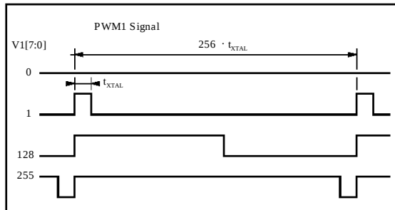
Figure 6 : PWM Timing
