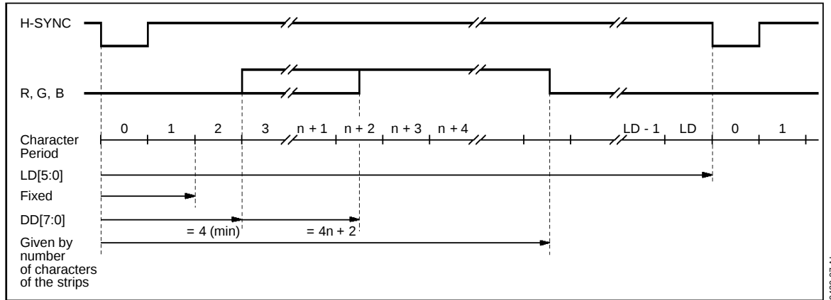
Figure 5 : Horizontal Timing
