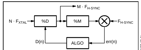
Figure 10 : Digital PLL
