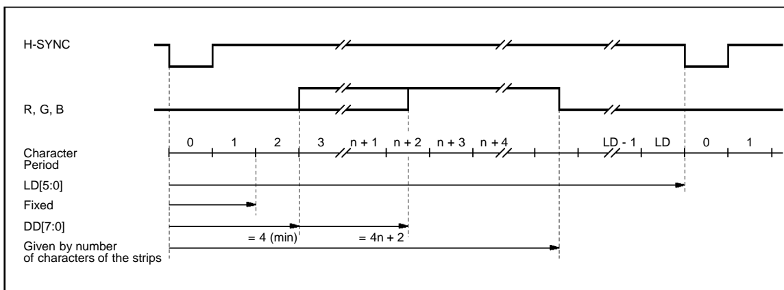
Figure 5 : Horizontal Timing
