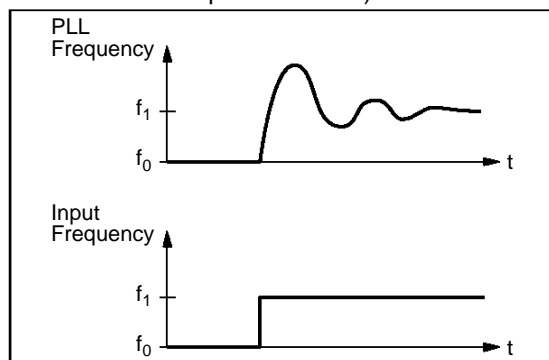
Figure 12 : Time Response of the PLL/Characteristic Equation Solutions (with Complex Solutions)
