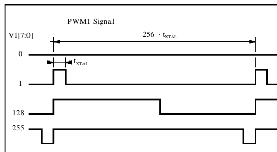
Figure 6 : PWM Timing
