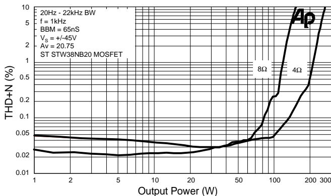
THD+N vs Output Power
