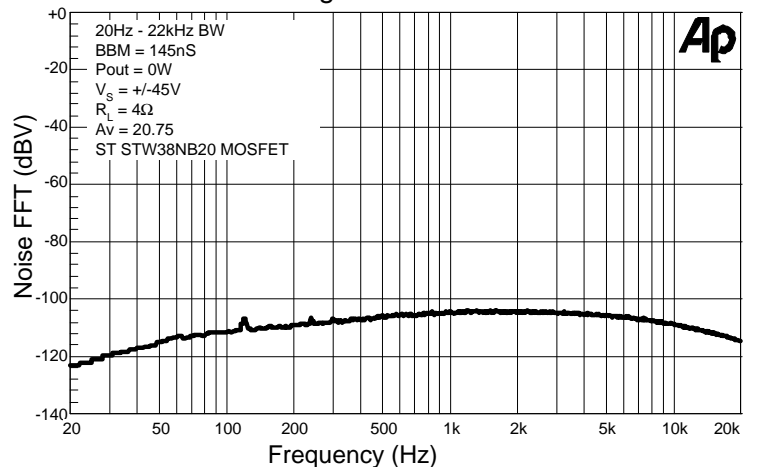
A-Weighted Noise FFT
