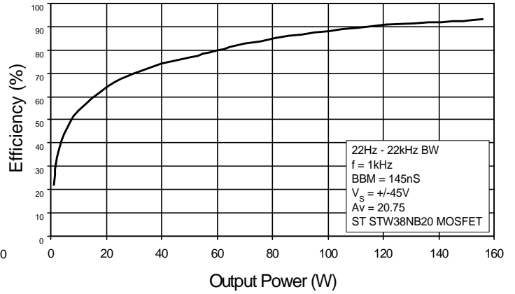
Efficiency versus Output Power R_L = 8\Omega
