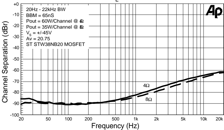
Channel Separation versus Frequency R_L = 4\Omega
