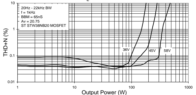
THD+N versus Output Power versus Supply Voltage R L = 4Ω
