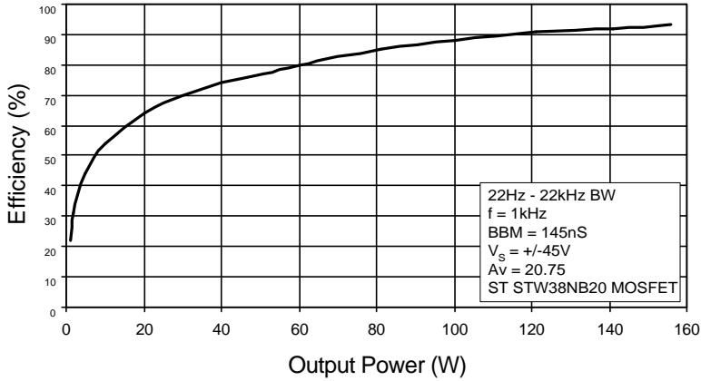
Efficiency versus Output Power R_L = 8\Omega
