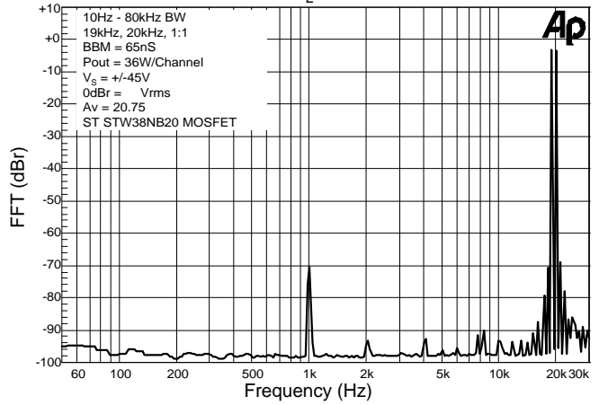
Intermodulation Performance R_L = 4\Omega
