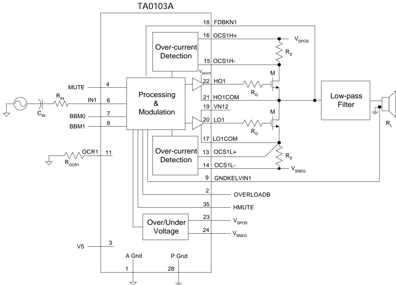
Figure 1. Simplified TA0103A Amplifier
