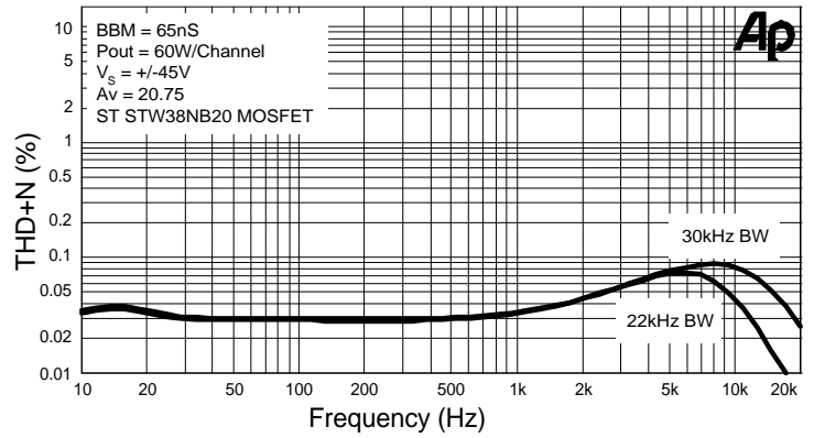
THD+N versus Frequency versus Bandwidth, R_L = 4\Omega
