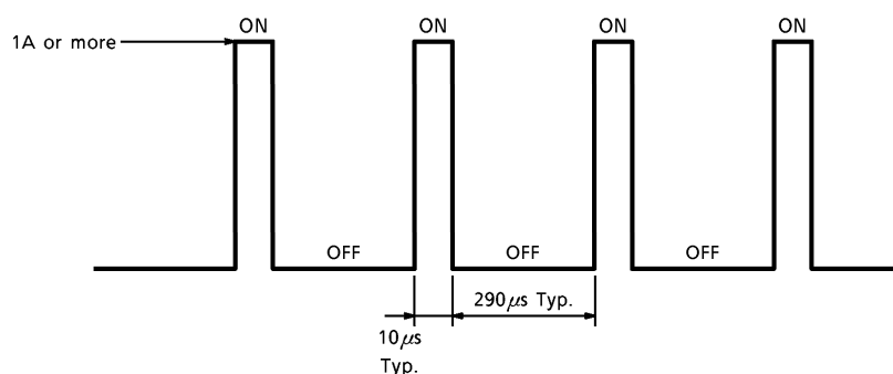
Fig.1 Basic Operation
