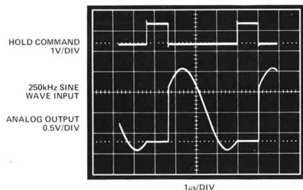
Figure 6c. Track/Hold Operation
