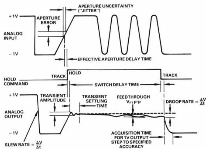
Figure 2. Track/Hold Waveforms
