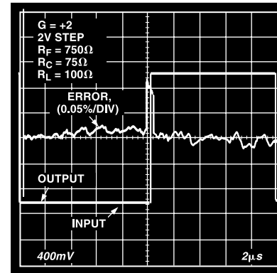
Figure 25. Long-Term Settling Time
