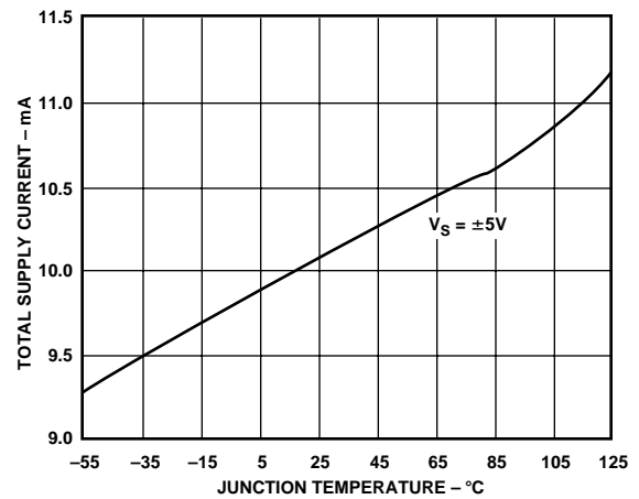
Figure 27. Total Supply Current vs. Temperature
