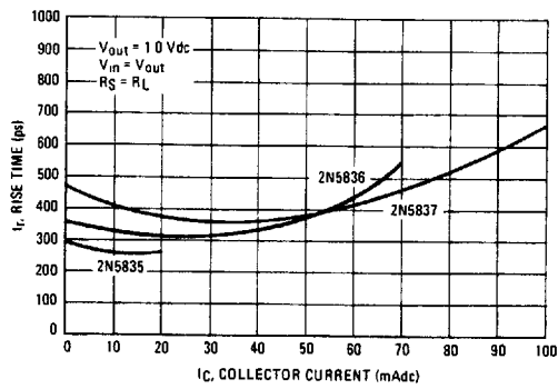
FIGURE 2 - SWITCHING TIME
