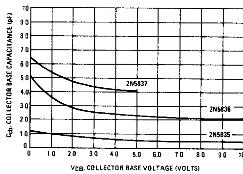
FIGURE 7 - COLLECTOR-BASE CAPACITANCE
