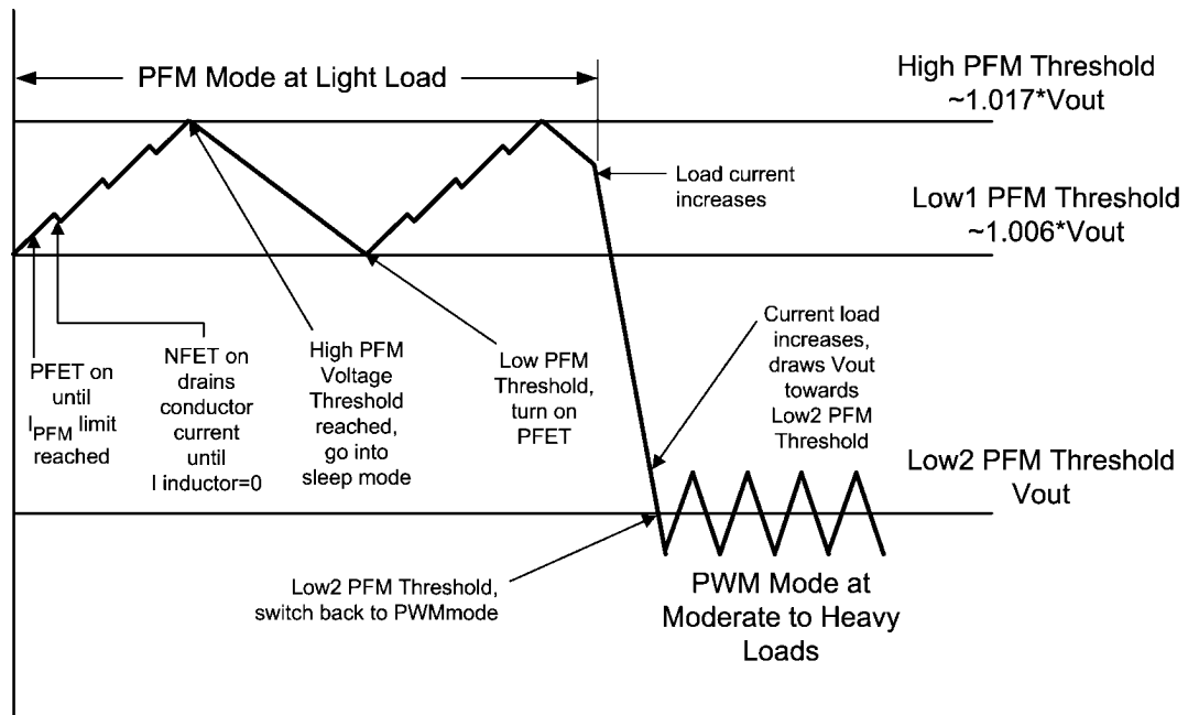
FIGURE 5. Typical PFM Operation
