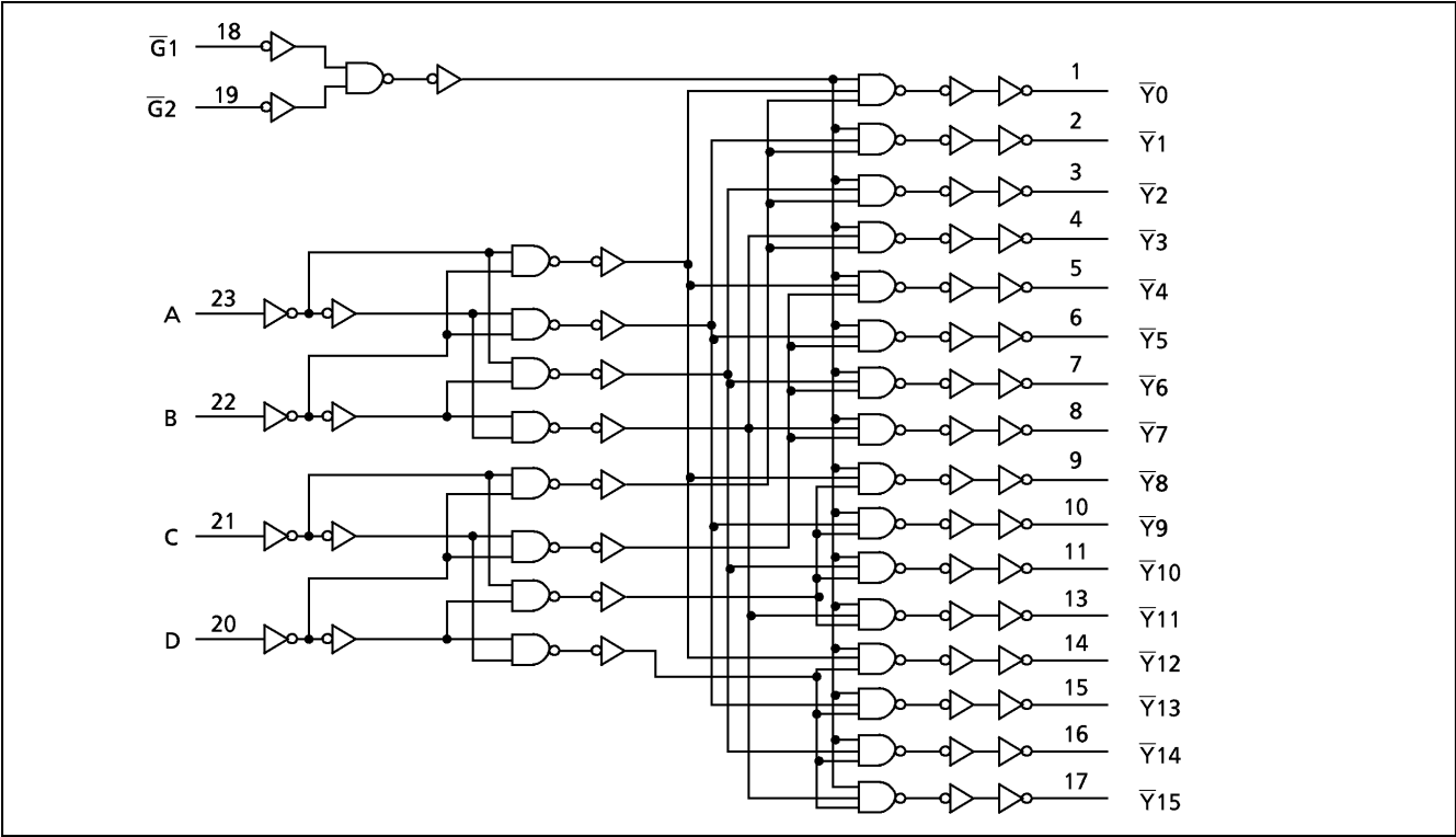
SYSTEM DIAGRAM
