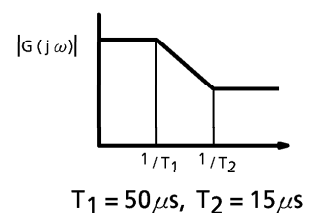
Fig.6 Filter characteristic
