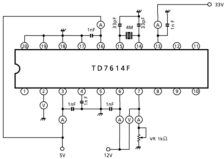
TEST CIRCUIT 1. Supply test circuit
