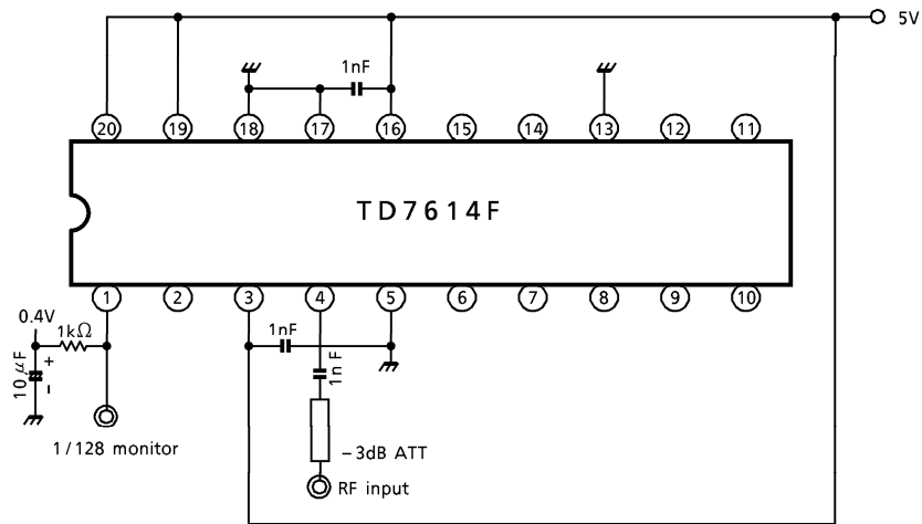
TEST CIRCUIT 4. Output mode test circuit
