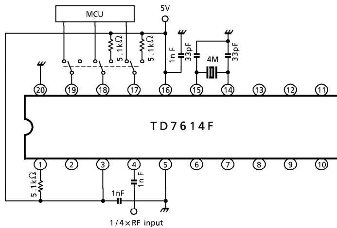
TEST CIRCUIT 4. Output mode test circuit
