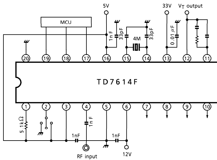
TEST CIRCUIT 2. AC operating test circuit
