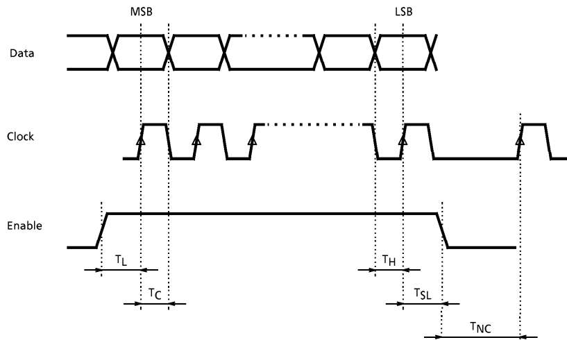
Fig.3 Timing chart of 3 wire-bus (rising timing)
