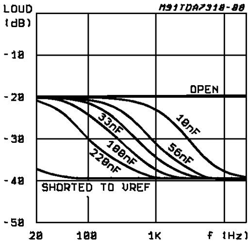
Figure 3: Loudness versus External Capacitors
