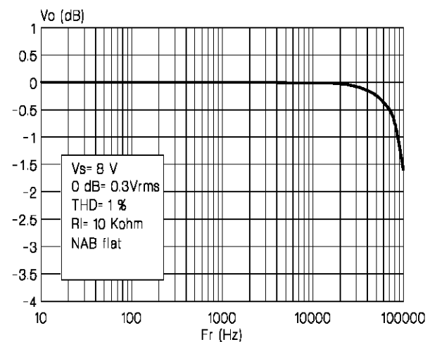
Figure 18: Power Bandwidth
