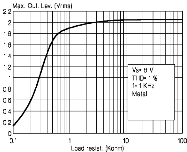
Figure 11: Load Characteristic
