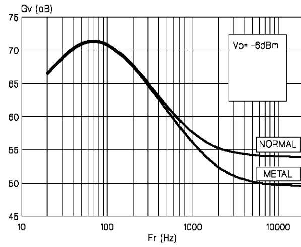
Figure 20: NAB Network
