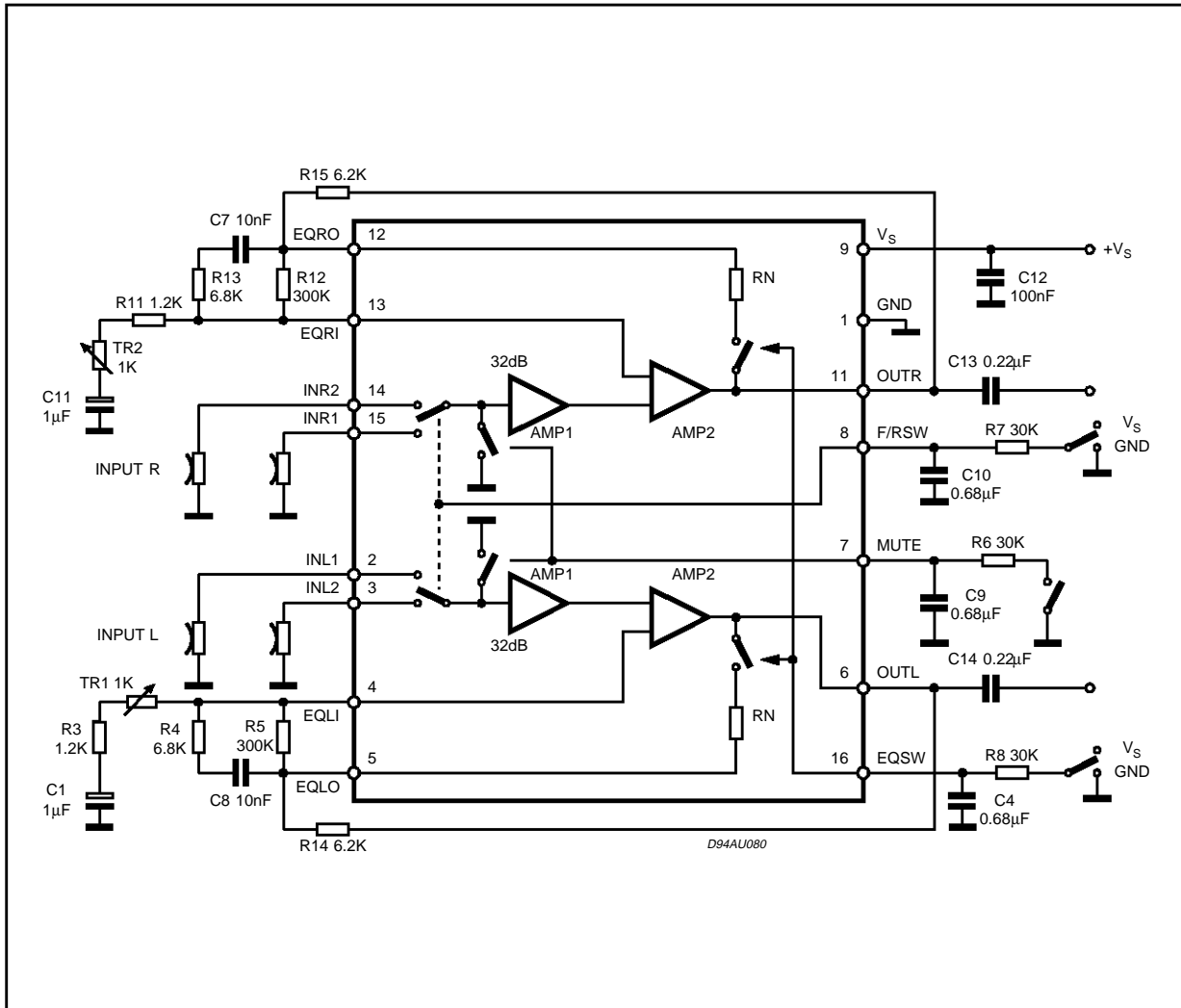
Figure 1: Application Circuit
