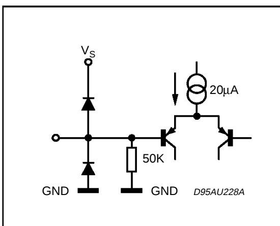
PIN: ADDR
