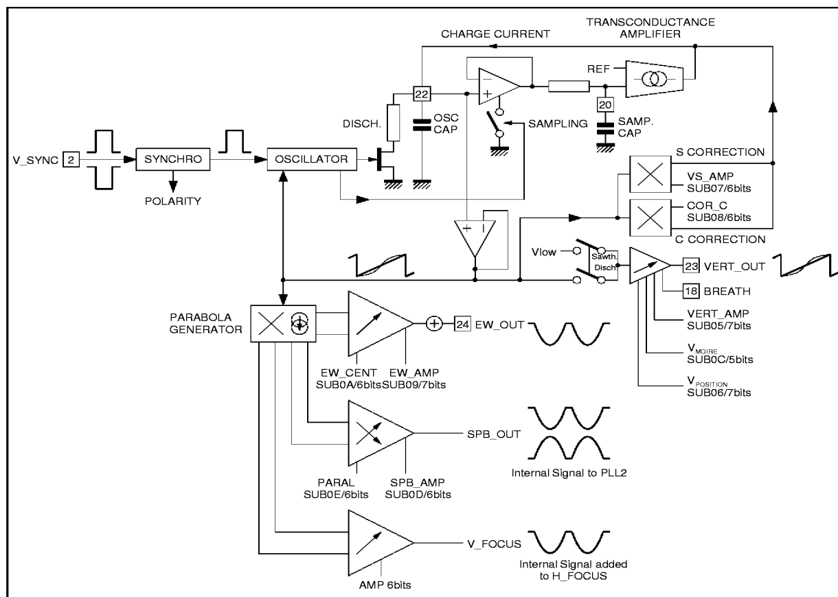
Figure 21 : Vertical Part Block Diagram
