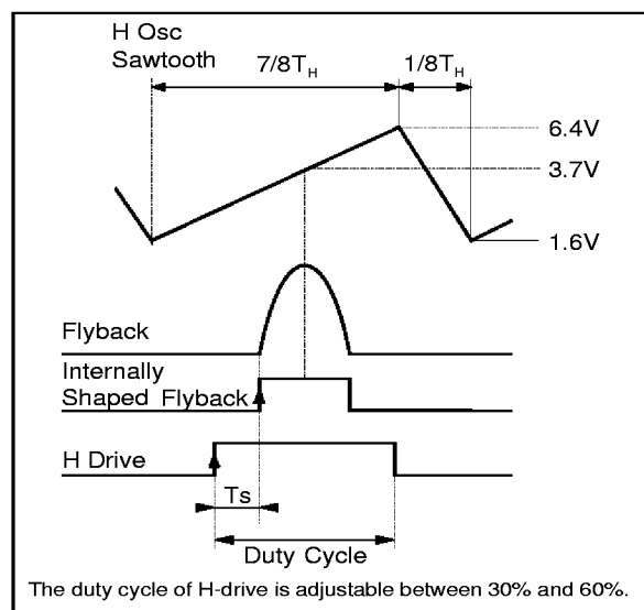
Figure 14 : Flyback Input Electrical Diagram
