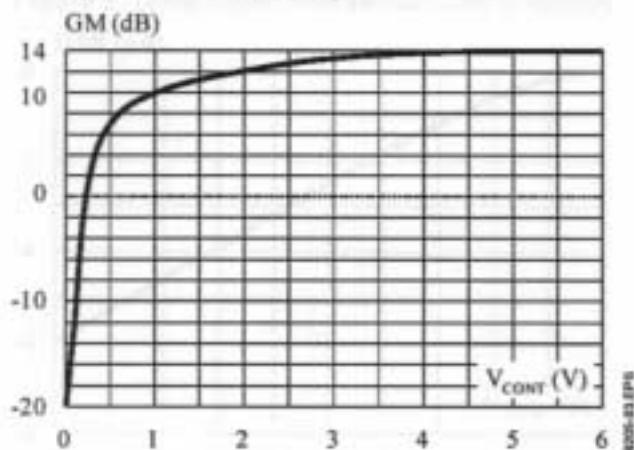
Figure 1 : Contrast Adjustment versus Control Voltage
