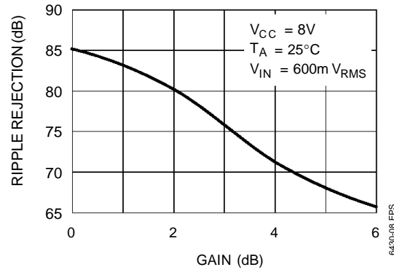
Figure 5 : Ripple Rejection as a Function of Gain
