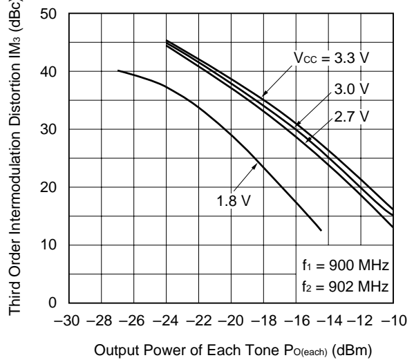
IM_3 - P_{O(each)}
