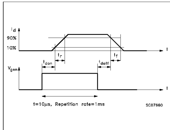
Fig. 6: Waveforms
