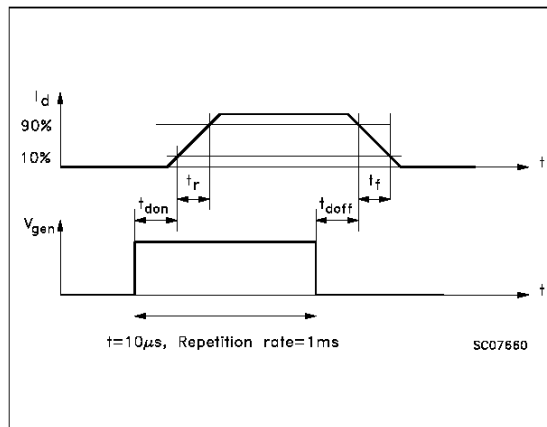
Fig. 6: Waveforms
