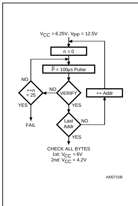
Figure 7. Programming Flowchart
