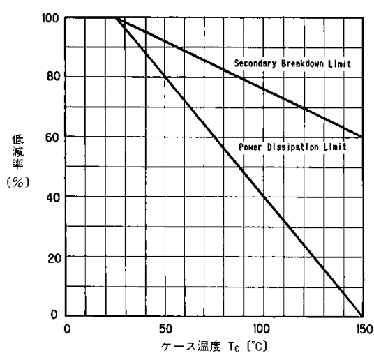
ASO Derating
