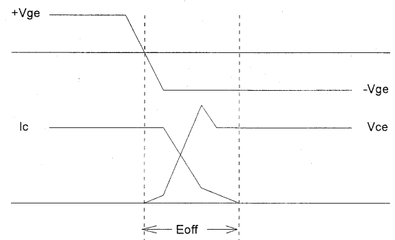
Turn-off Waveforms
