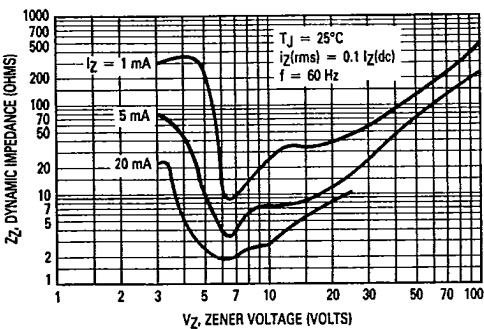
Figure 9. Effect of Zener Voltage on Zener Impedance
