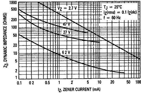
Figure 8. Effect of Zener Current on Zener Impedance
