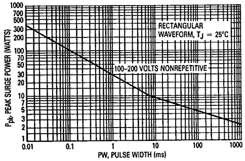
Figure 7b. Maximum Surge Power DO-204AH 100-200 Volts
