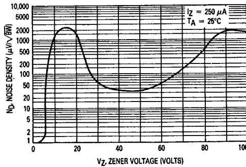
Figure 10. Typical Noise Density
