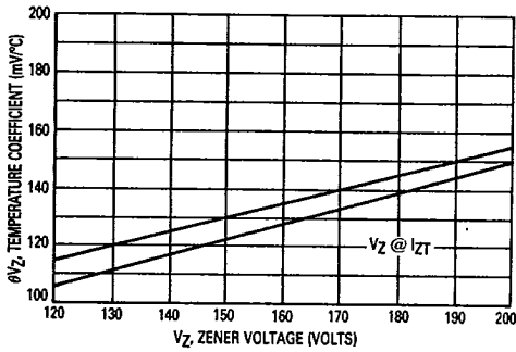
Figure 4c. Range for Units 120 to 200 Volts
