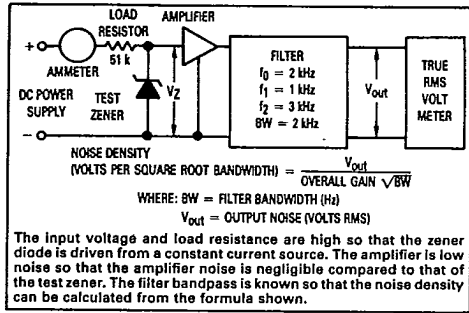
Figure 11. Noise Density Measurement Method
