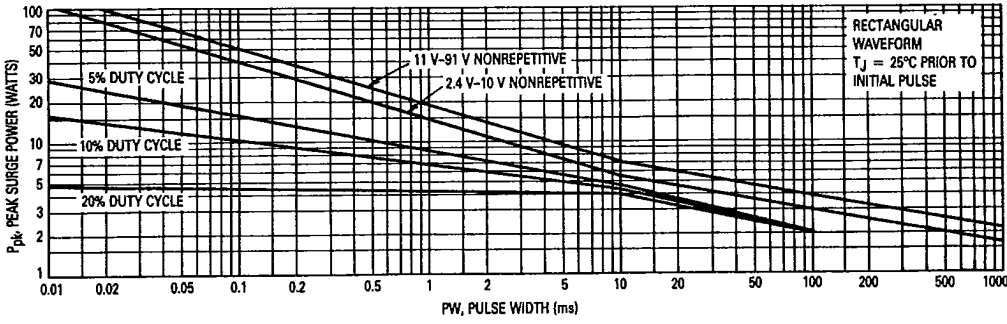
Figure 7a. Maximum Surge Power 2.4-9 Volts
