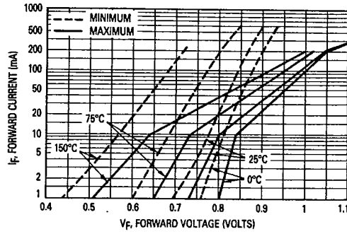
Figure 12. Typical Forward Characteristics
