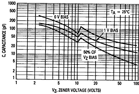
Figure 6a. Typical Capacitance 1-100 Volts
