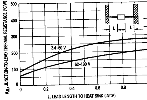
Figure 2. Typical Thermal Resistance
