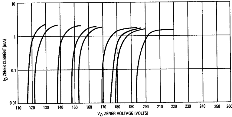
Figure 16. Zener Voltage versus Zener Current — V_Z = 110 -220 Volts
