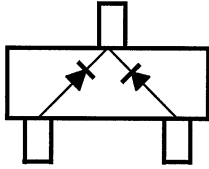
Equivalent Circuit (Top View)
