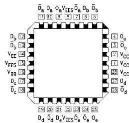
28-Pin PLCC
