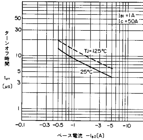
I b2 依存性特性 I b2 Dependence of Turn off Time
