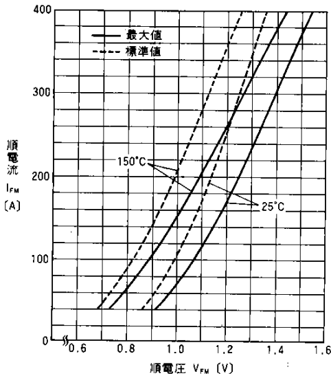
順特性 Forward Characteristics
