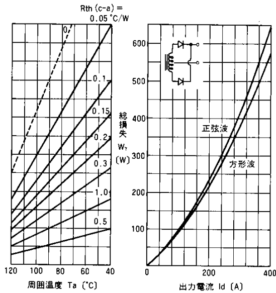
総損失-出力電流-周囲温度 Power Loss-Output Current-Ambient Temperature
