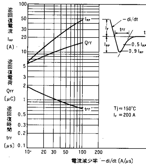
逆回復特性 Reverse Recovery Characteristics
