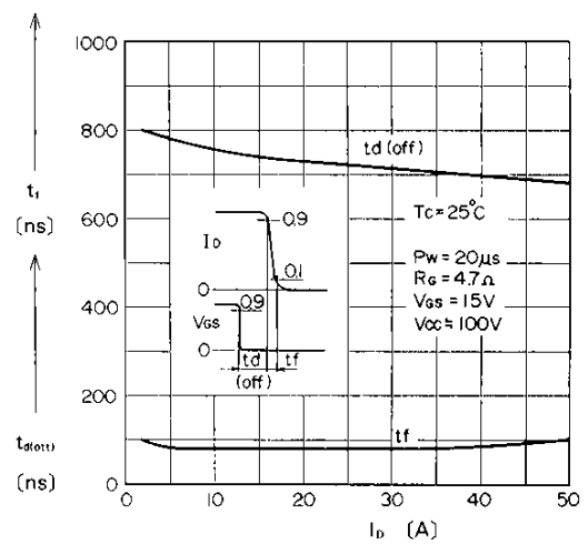
Turn-OFF Characteristics
