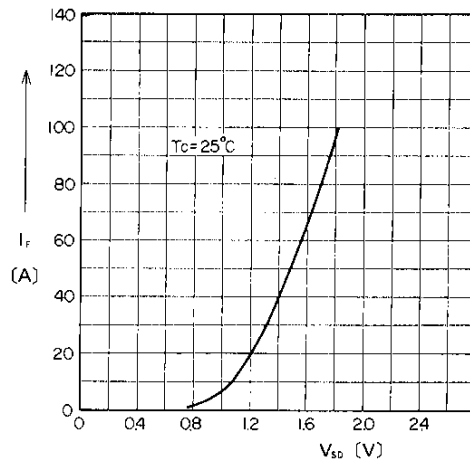
Forward Voltage of FWD
