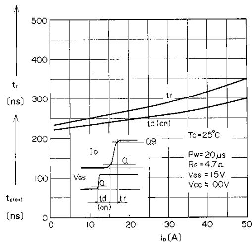
Turn-ON Characteristics
