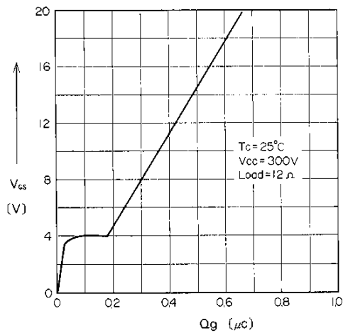
Typical Input Charge
