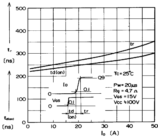
Turn-ON Characteristics
