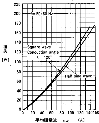
総損失—出力電流 Power Loss—Output Current
