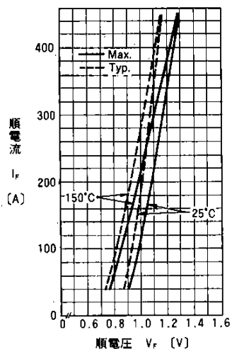
順特性 Forward Characteristics
