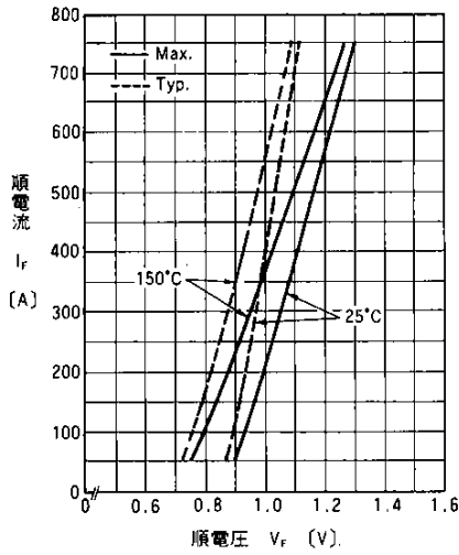
順特性 Forward Characteristics
