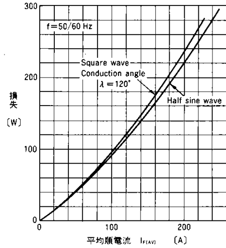
総損失—出力電流 Power Loss—Output Current
