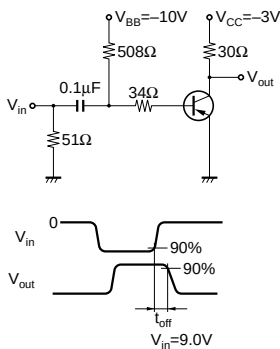
t_{stg} Test Circuit
