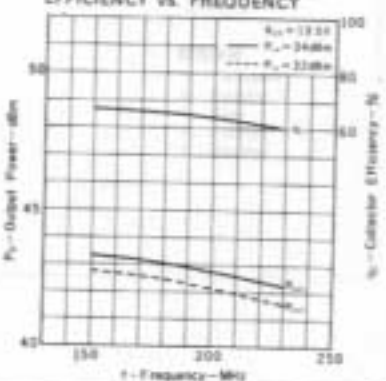
OUTPUT POWER & COLLECTOR EFFICIENCY vs. FREQUENCY
