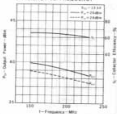
OUTPUT POWER & COLLECTOR EFFICIENCY vs. FREQUENCY
