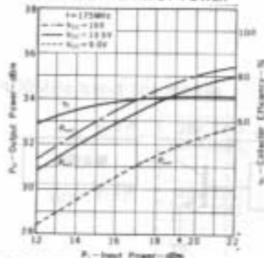
OUTPUT POWER & COLLECTOR EFFICIENCY vs. INPUT POWER
