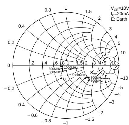
S_{11}, S_{22}
